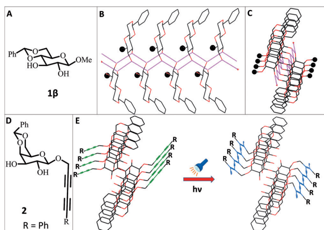
Figure 2. A) Structure of methyl 4,6- O -benzylidene-β-D-glucopyranoside ( 1β ). B) Crystal packing of 1β showing hydrogen-bonded 1D assembly. C) View of hydrogen-bonded 1D assembly along the direction of hydrogen bonding showing the stacking of methyl groups. D) Chemical structure of photo-polymerizable organogelator 2 . E) Representation of the molecular packing arrangement in gel state and subsequent topochemical polymerization of monomeric gelator 2 .
